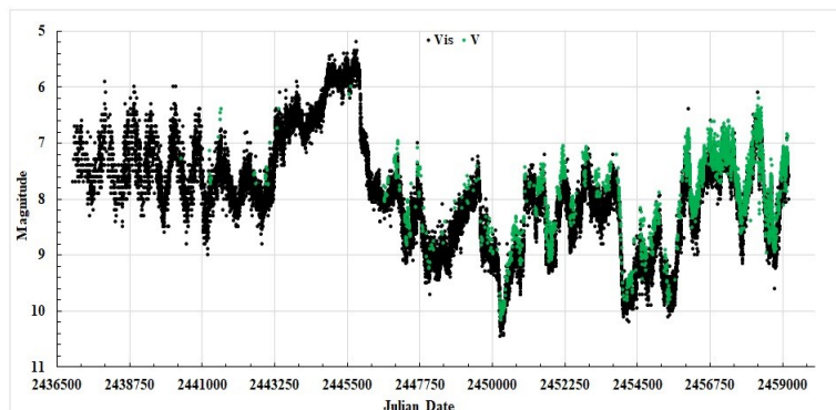
Fig. 1. Light curve of the symbiotic star CH Cyg for the period 1963-2021, according to AAVSO.
