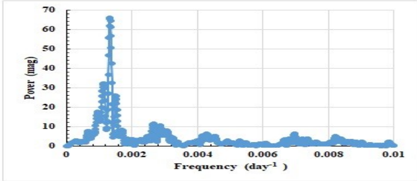
Fig. 7. Power spectrum built in frequency ranges 0-0.01 for the V value array.
