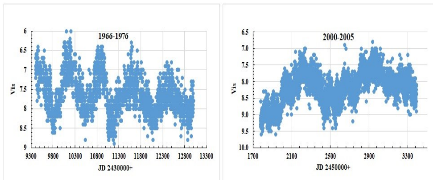
Fig. 3. Light curve of the symbiotic star CH Cyg (based on AAVSO observations) for the periods 1966-1976 and 2000-2005.
