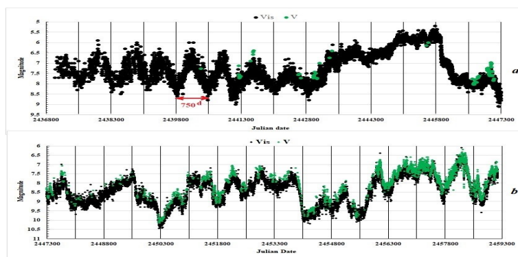
Fig. 2. Light curve for the period 1963-2021, according to AAVSO. a) 1963-1988, b) 1988-2021.
