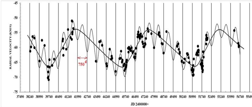
Fig. 5. JD-dependent curve of the general view of the radial velocity curve of the absorption line of the symbiotic star CH Cyg. (In the figure 2438240-2441990 is the result of Deutsch measurements, 2443490-2448740 period Hinkle measurements, 2448490-2452490 period Ijima and Mikayilov measurements, 2453990- 2454740 period Mikailov measurements).
