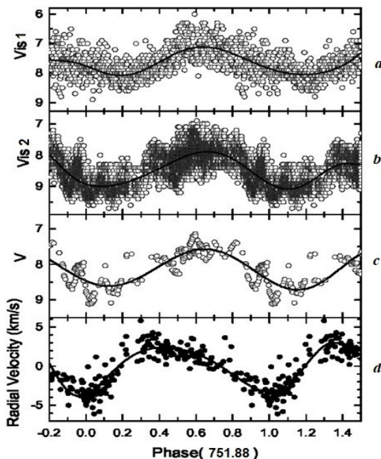
Fig. 8. Phase diagram of star size and radial velocities of absorption lines.
