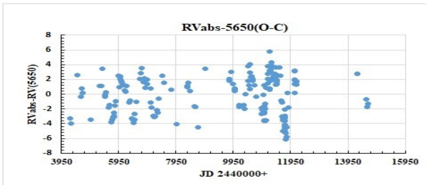
Fig. 6. Long-term velocity is subtracted from each observed velocity.
