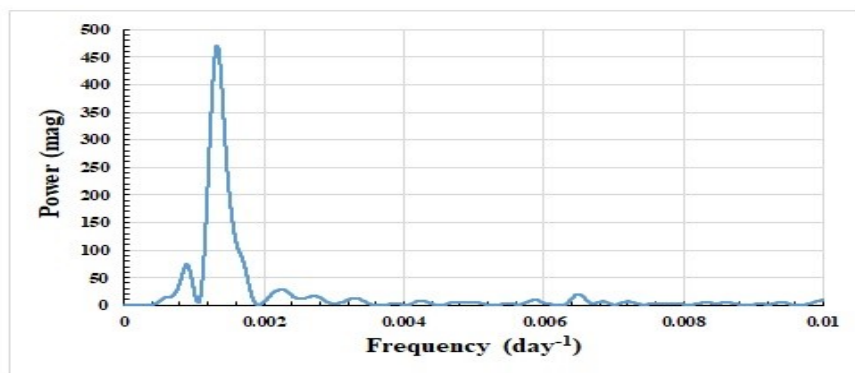
Fig. 4. Power spectrum built in the frequency range 0-0.01 for the V value array.
